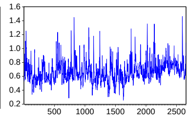
DCC BETA P9
