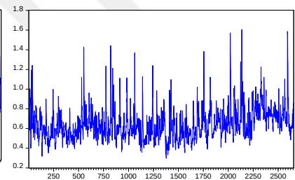
DCC BETA (P18)
